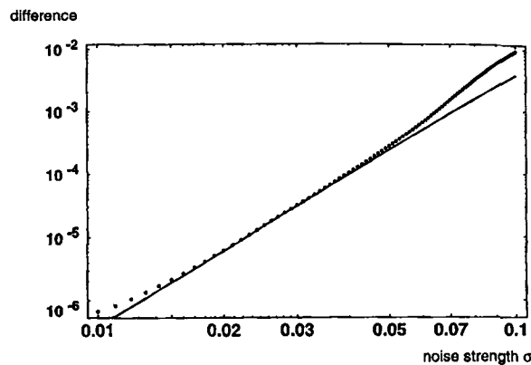
Fig. 1. The deviation of the analytic estimate (44) from the numerically computed \nu_0(\sigma) for a range of values of the noise strength \sigma (points), vs. the conjectured remainder, 38\sigma^4 (solid line). For small \sigma the errors are due to the finiteness of the grid, and for larger \sigma the deviations is due to the neglected higher order contributions.
