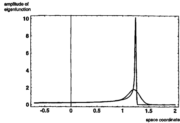
Fig. 2. The eigenfunction for \sigma = 0.01 (sharp peak) and \sigma = 0.1 (smoother).
